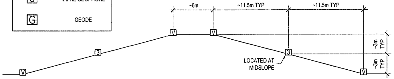
1 TYPICAL CROSS SECTION 1/8" = 1m
